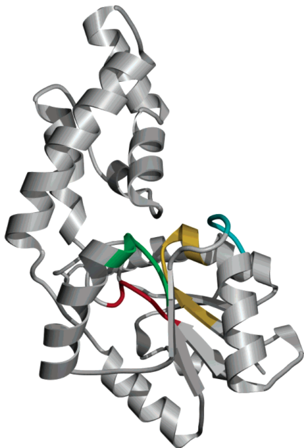
FIGURE 2: Phosphonatase structure (4) depicted as a ribbon diagram with catalytic loops colored as follows: red for loop 1, green for loop 2, cyan for loop 3, and gold for loop 4.
